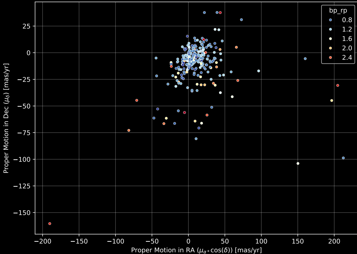
APOGEE DR17 Field: [120-85] Proper Motion Diagram (n= 259)
