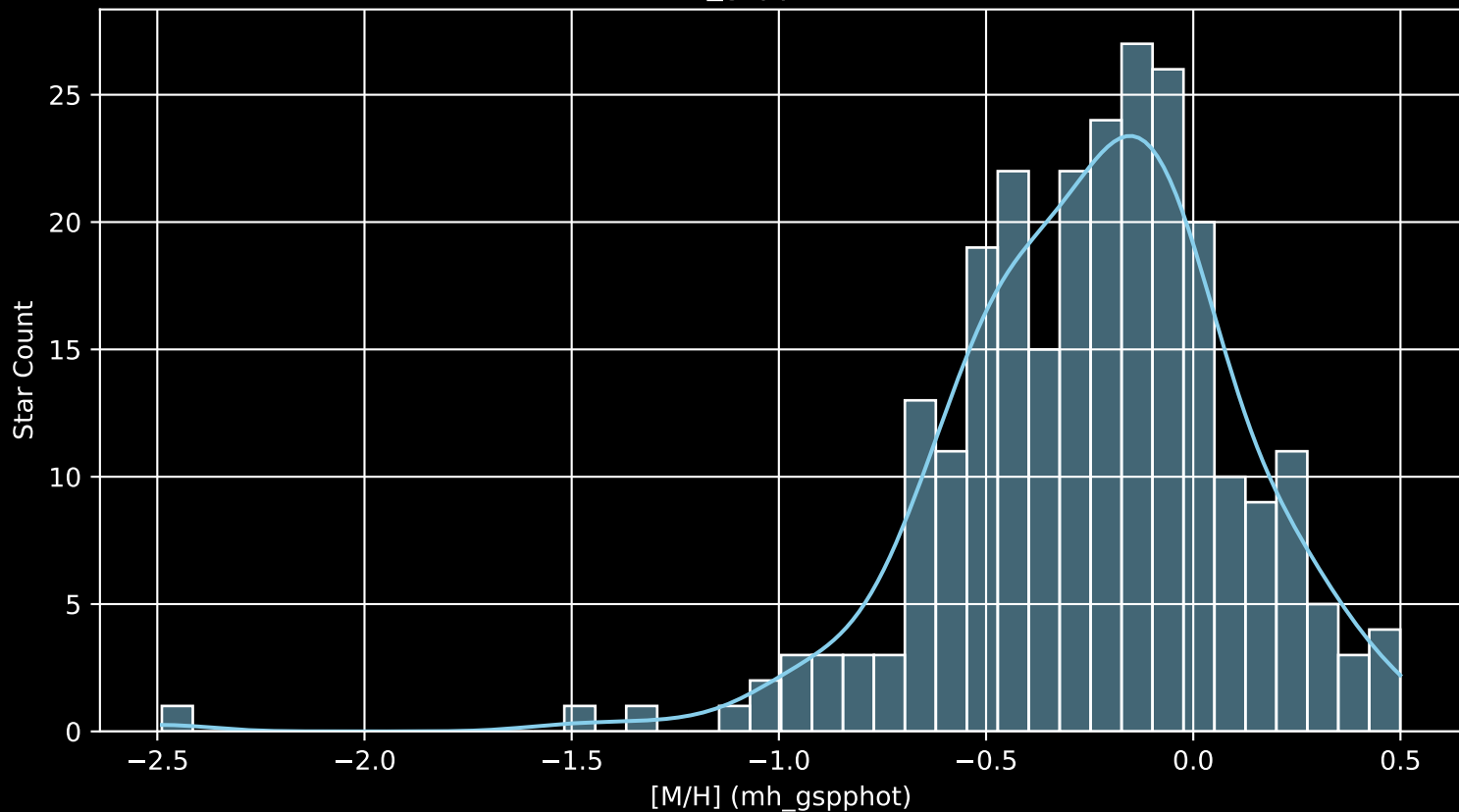
APOGEE DR17 Field: [120-85 [M/H] (mh_gspphot) (n= 259)
