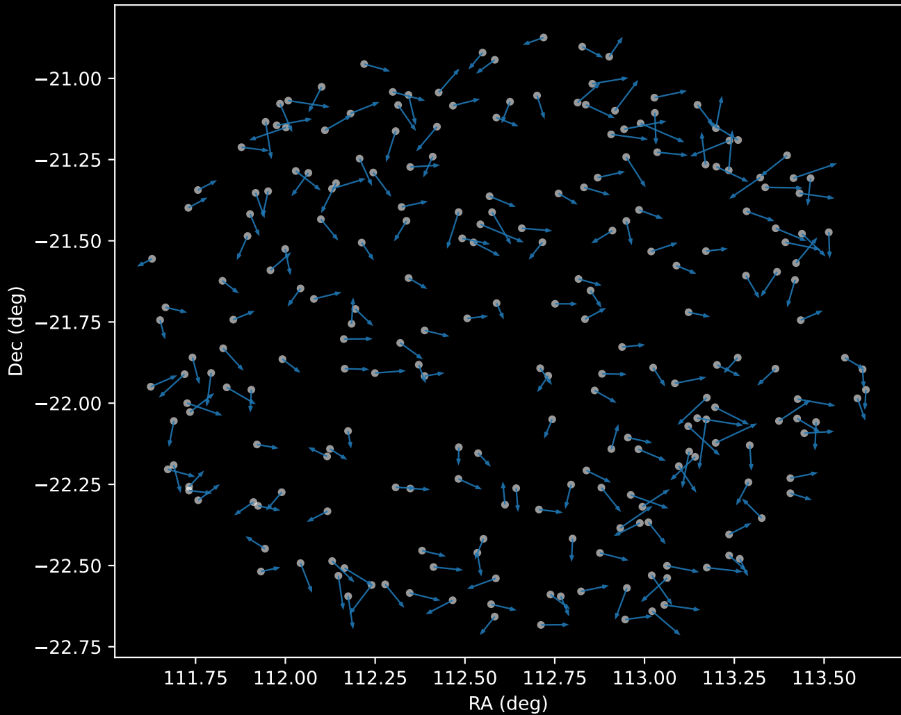
APOGEE DR17 Cluster 0 Proper Motion Vectors (n=232)
