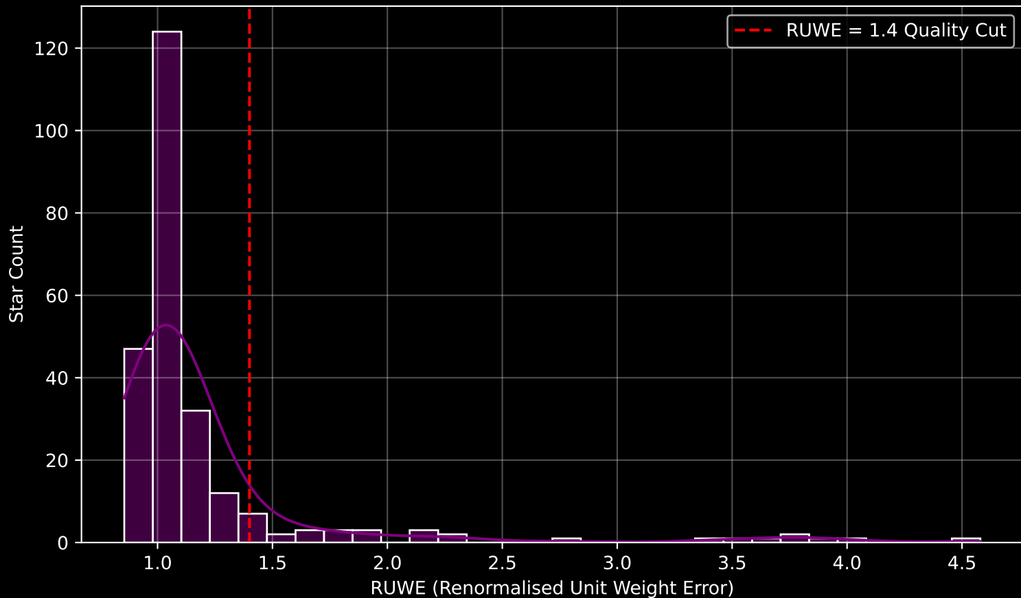
GAPOGEE DR17 Field [120-85] RUWE Distribution (n= 247)
