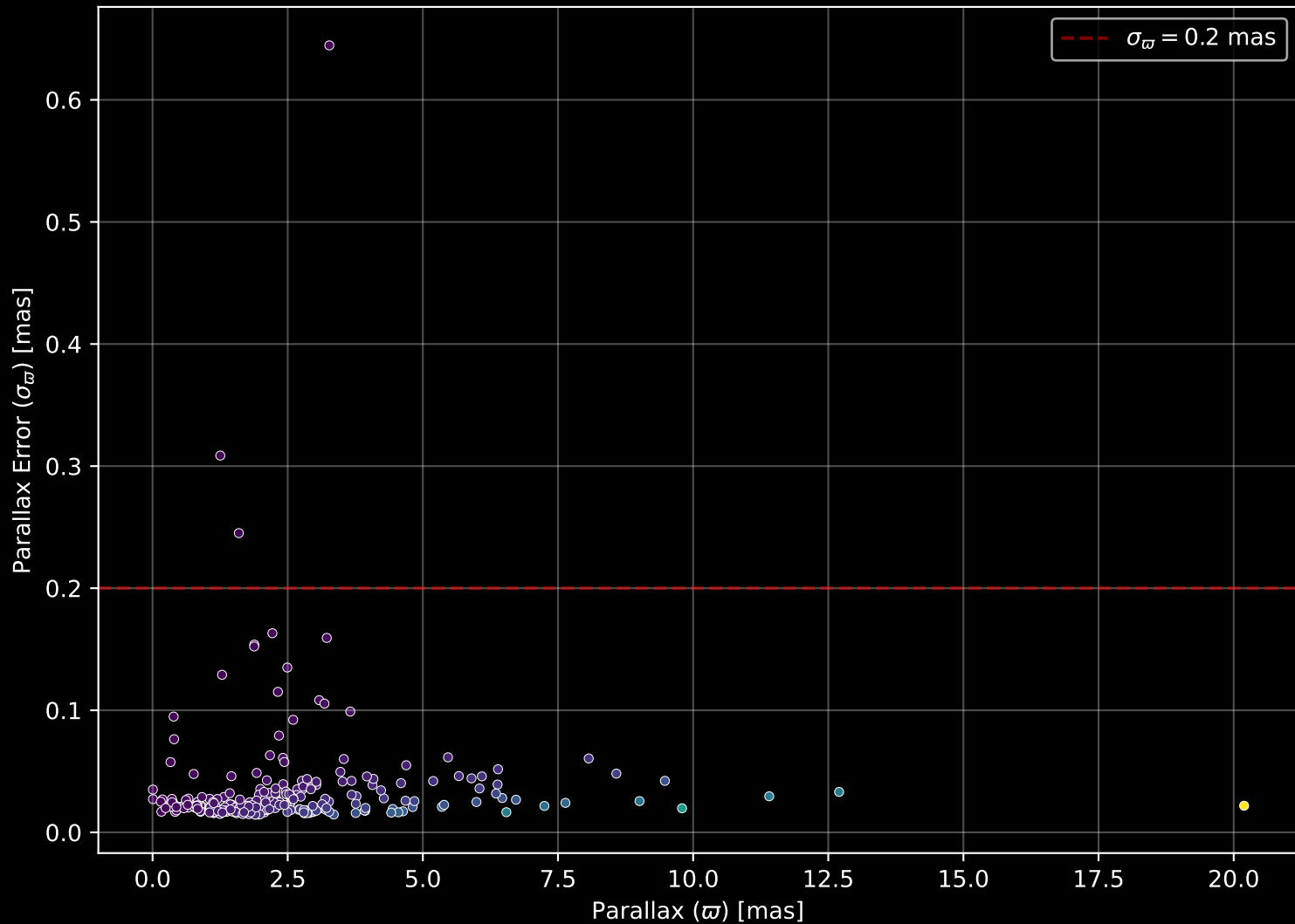
APOGEE DR17 Field: [120-85] Parallax Quality (n= 259)
