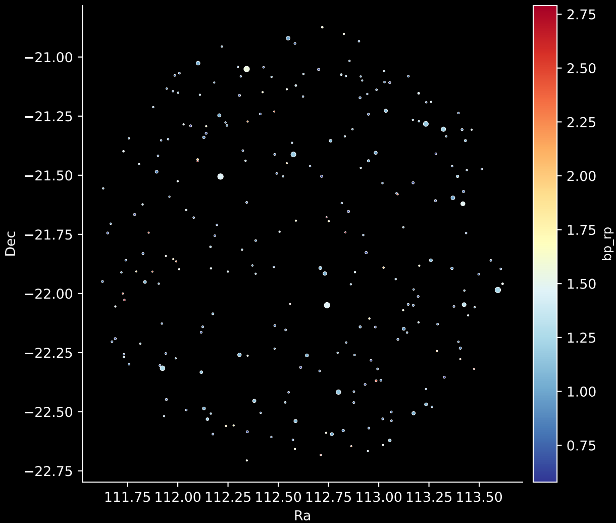
APOGEE DR17 Field: [120-85] Stars: 259
