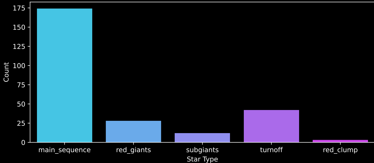
APOGEE DR17 Field: [120-85] Count plot of Star Type
